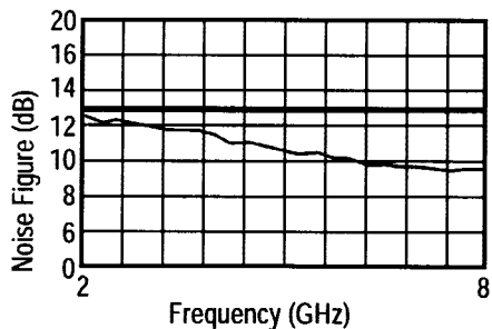
Figure 7. Noise Figure vs. Frequency
