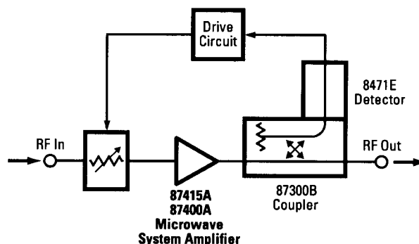
Figure 1. External leveling looping
