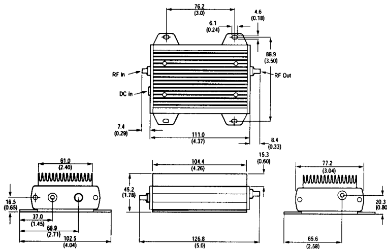
Figure 2. Agilent 87415A outline drawing. Dimensions in millimeters and (inches).
