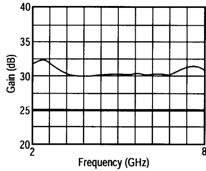
Figure 5. Gain vs. Frequency
